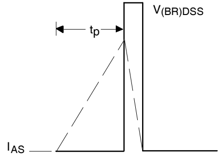
Fig 22b. Unclamped Inductive Waveforms
