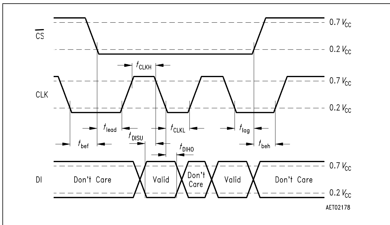
Figure 11 SPI-Input Timing
