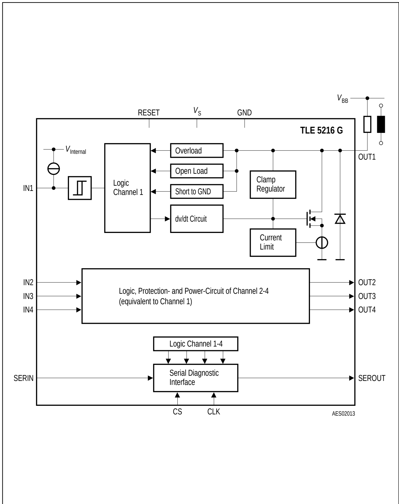
Figure 2 Block Diagram
