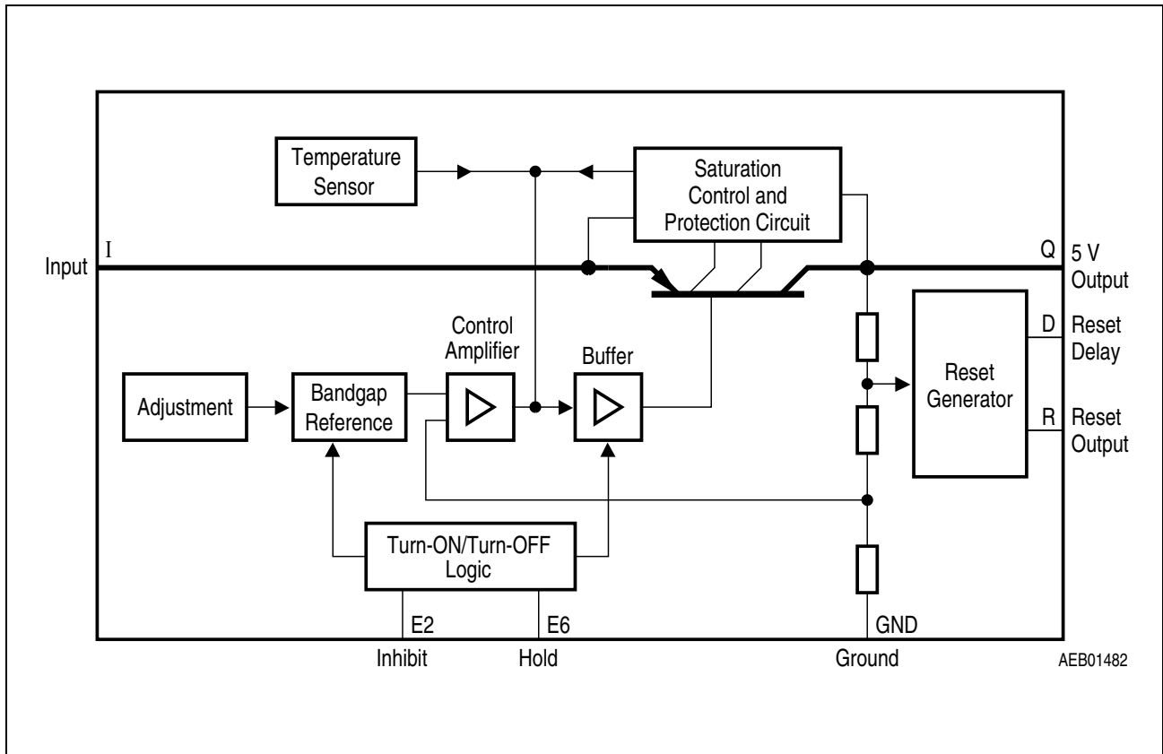
Figure 3 Block Diagram
