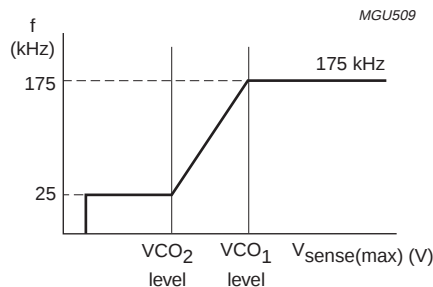
Fig.7 VCO frequency as function of V_{sense(max)} .
