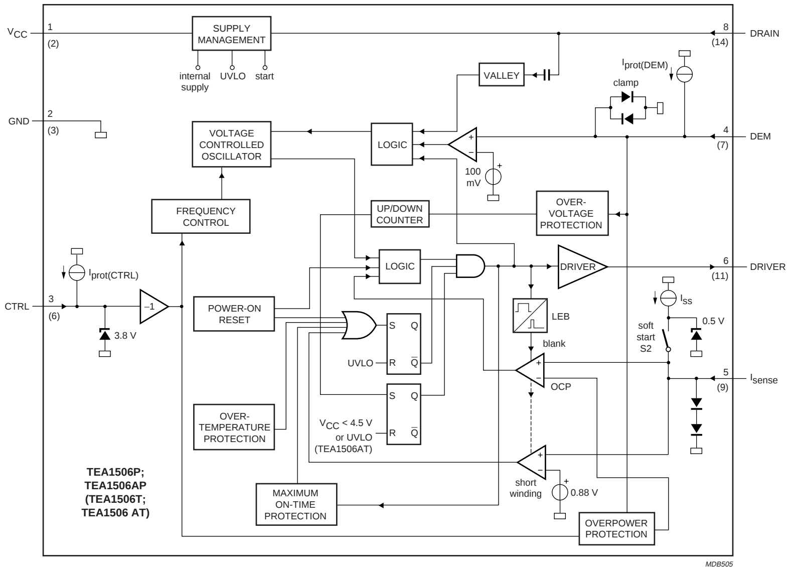
Fig.2 Block diagram.
