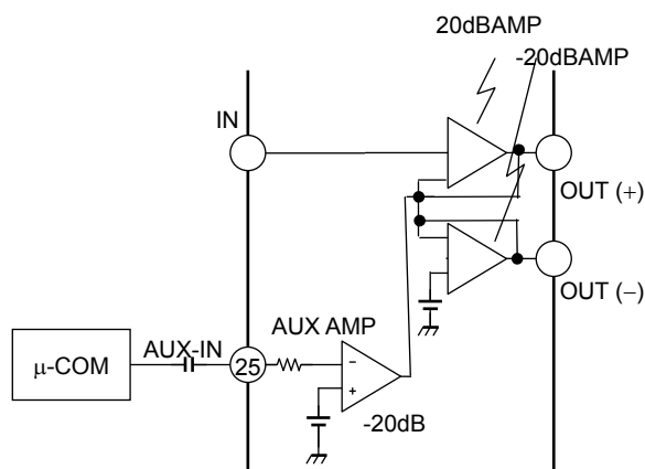
Figure 5 AUX IN
