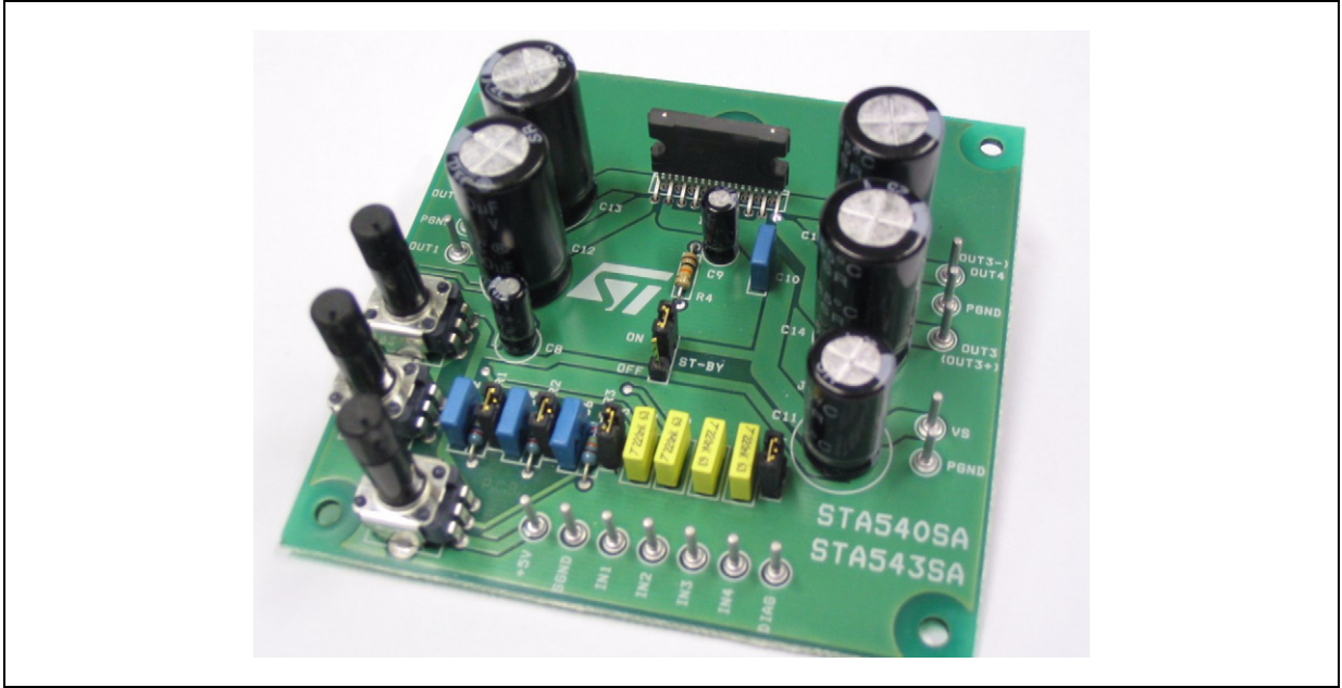
Figure 3. Test board
