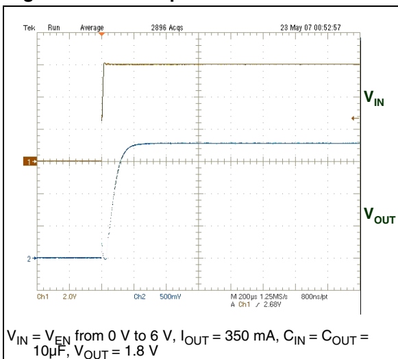
Figure 24. Start-up transient
