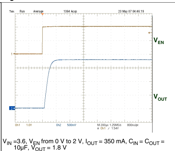
Figure 25. Enable transient
