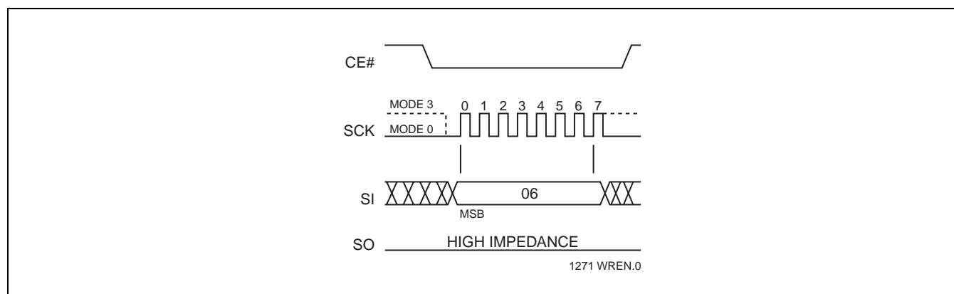
FIGURE 16: WRITE ENABLE (WREN) SEQUENCE
