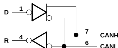
SN65HVD232Q Logic Diagram (Positive Logic)
