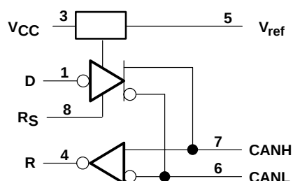
SN65HVD230Q, SN65HVD231Q Logic Diagram (Positive Logic)
