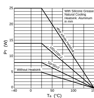
Pr-Ta Characteristics
