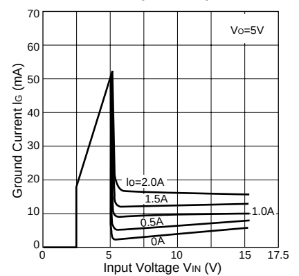
Circuit Current(SI-3052V)
