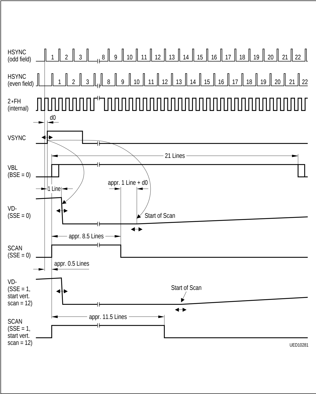
Figure 9 Timing Diagram of SCAN if STE = 0
