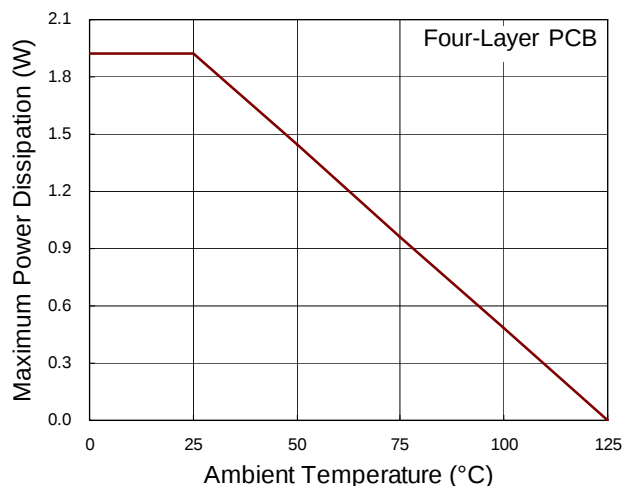
Figure 5. Derating Curve for the RT8223L/M Package
