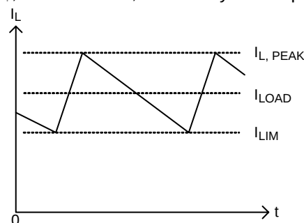
Figure 2. "Valley" Current-Limit
