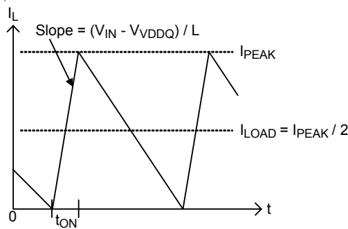
Figure 5. Boundary Condition of CCM/DCM
