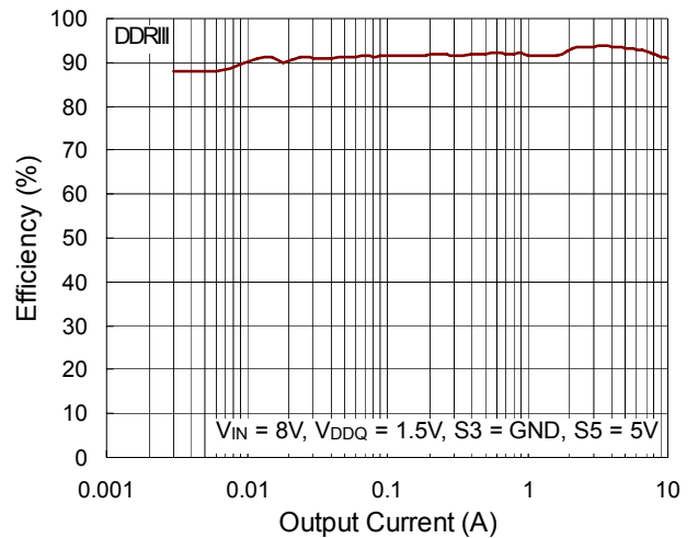
VDDQ Efficiency vs. Output Current
