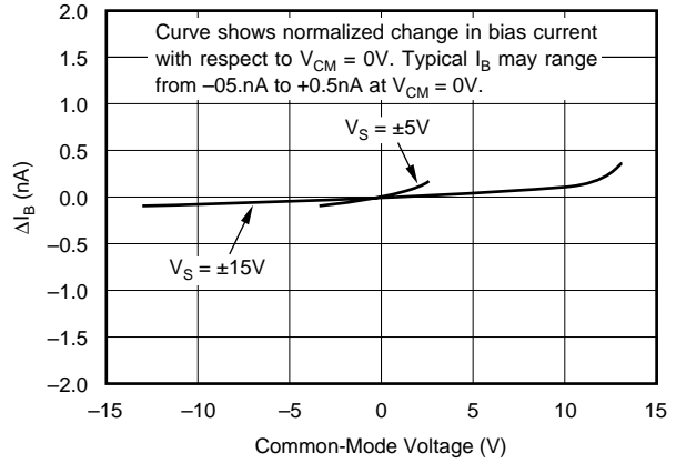
CHANGE IN INPUT BIAS CURRENT vs COMMON-MODE VOLTAGE
