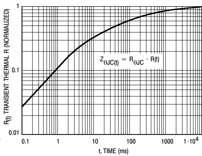
Figure 4. Transient Thermal Response
