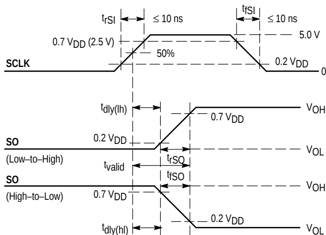
Figure 5. Valid Data Delay Time and Valid Time Waveforms
