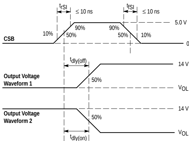
Figure 9. Turn-On/Off Waveforms
