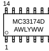
SO-14 D SUFFIX CASE 751A
