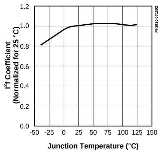
Figure 20. I^2f Coefficient vs. Temperature.
