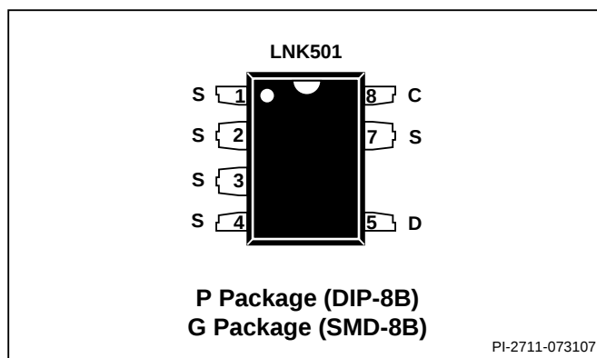
Figure 3. Pin Configuration.
