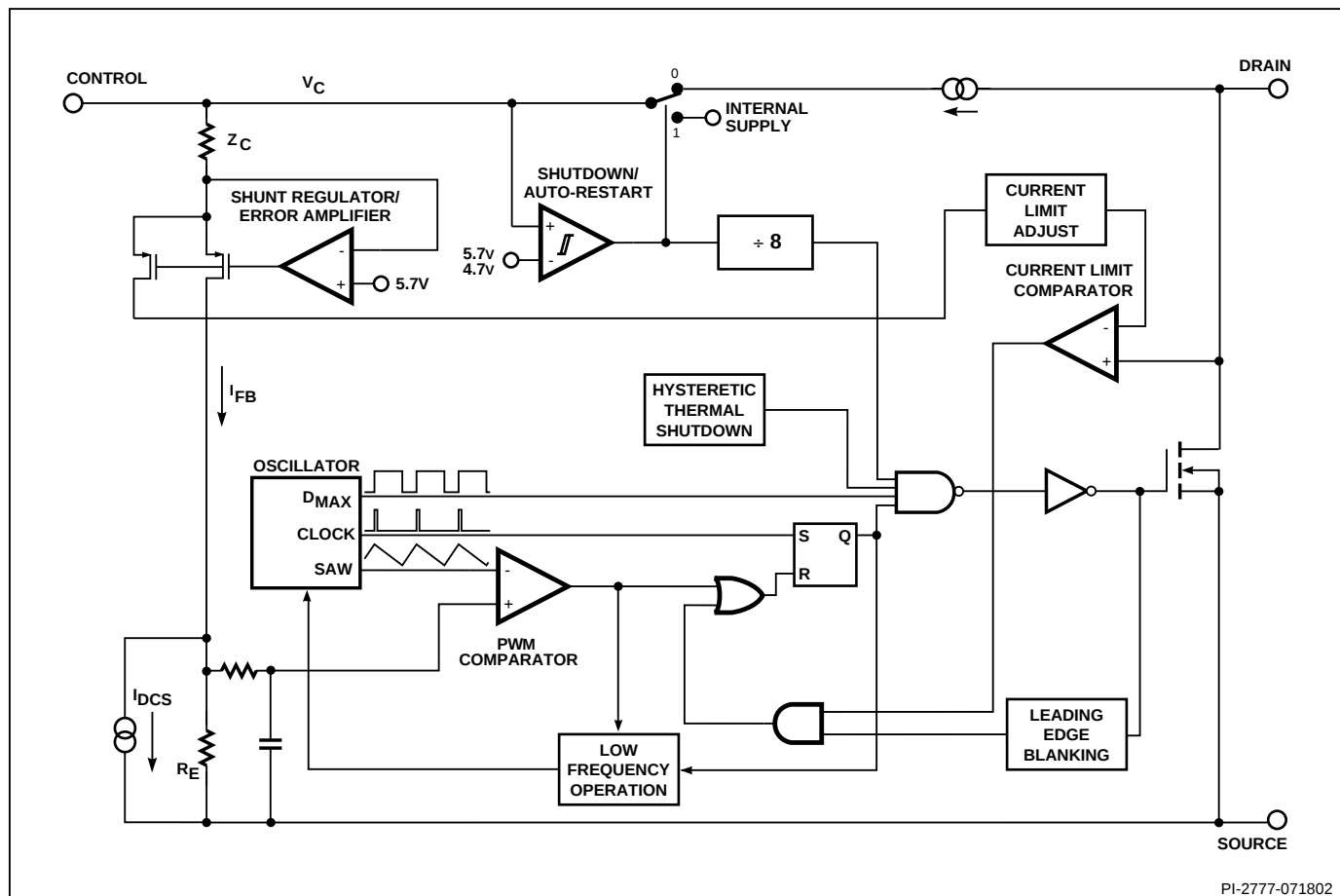
Figure 2. Block Diagram.
