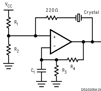
FIGURE 5. Crystal Oscillator
