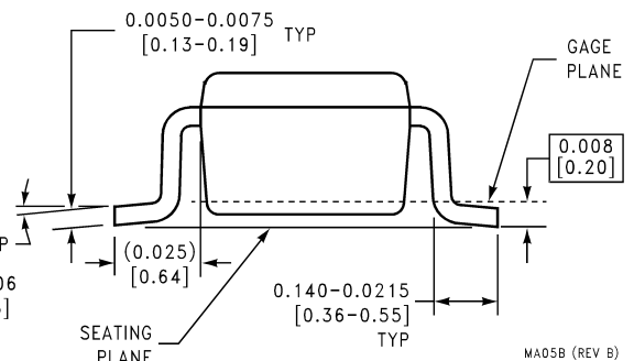
5-Pin SOT23-5 Tape and Reel Order Numbers LMV7219M5 or LMV7219M5X NS Package Number MA05B
