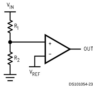
FIGURE 4. Threshold Detector
