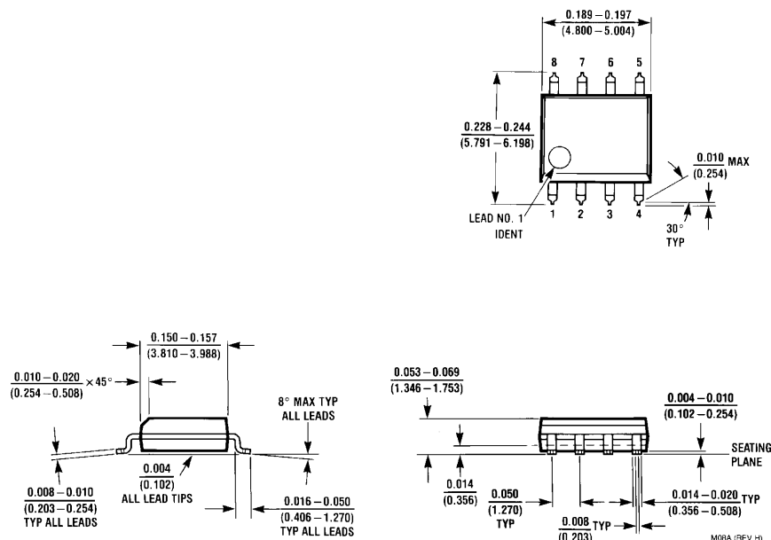
8-Pin Small Outline Package Order Number LM7301IMX NS Package Number M08A
