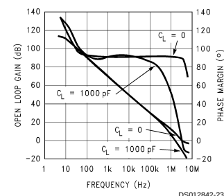
Gain and Phase, 2.7V Supply
