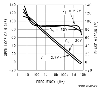
Gain and Phase
