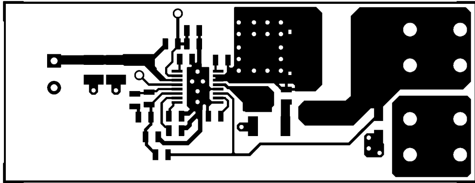
Component Side
