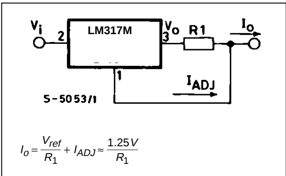
Figure 7 : Current Regulator.
