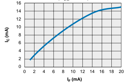
LDA210/LDA211 Typical Collector Current vs. Forward Current ( V_{CE} = 0.8V )
