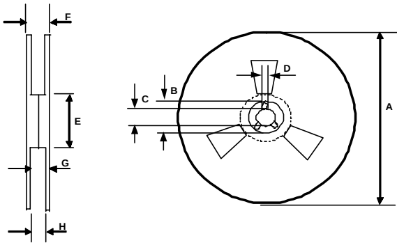
REEL DIMENSIONS FOR 8SOIC
