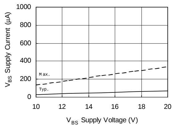
Figure 14B. V_{BS} Supply Current vs. Supply Voltage
