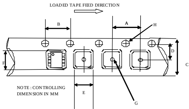
CARRIER TAPE DIMENSION FOR 8SOIC
