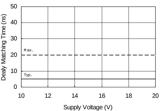
Figure 7B. Turn-off Delay Matching Time vs. Supply Voltage
