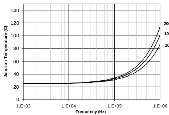
Figure 28. IR2010 Tj vs Frequency R GATE = 10 Ohm, V CC = 15V with IRFBC40
