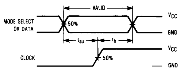
Figure 4. Switching Waveforms
