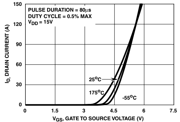
FIGURE 8. TRANSFER CHARACTERISTICS
