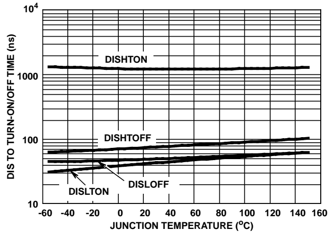
FIGURE 13. UPPER/LOWER DIS(ABLE) TO TURN-ON/OFF vs TEMPERATURE
