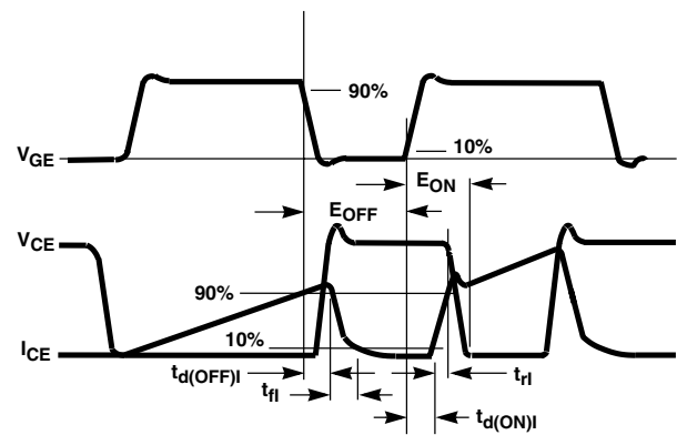
FIGURE 18. SWITCHING TEST WAVEFORM
