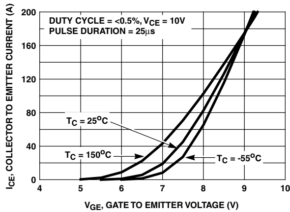
FIGURE 13. TRANSFER CHARACTERISTIC
