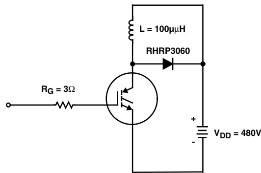
FIGURE 17. INDUCTIVE SWITCHING TEST CIRCUIT
