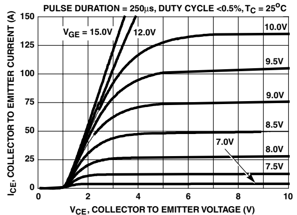
FIGURE 2. SATURATION CHARACTERISTICS
