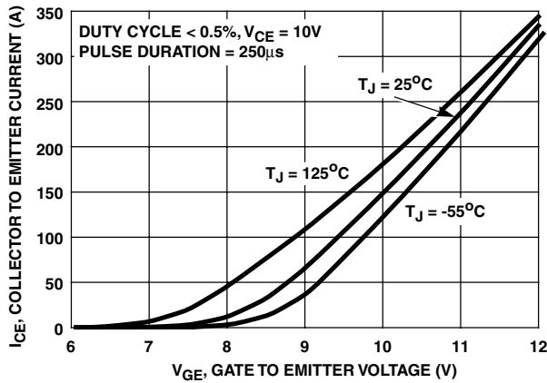
FIGURE 13. TRANSFER CHARACTERISTIC
