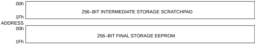
DS2430A MEMORY MAP Figure 5
