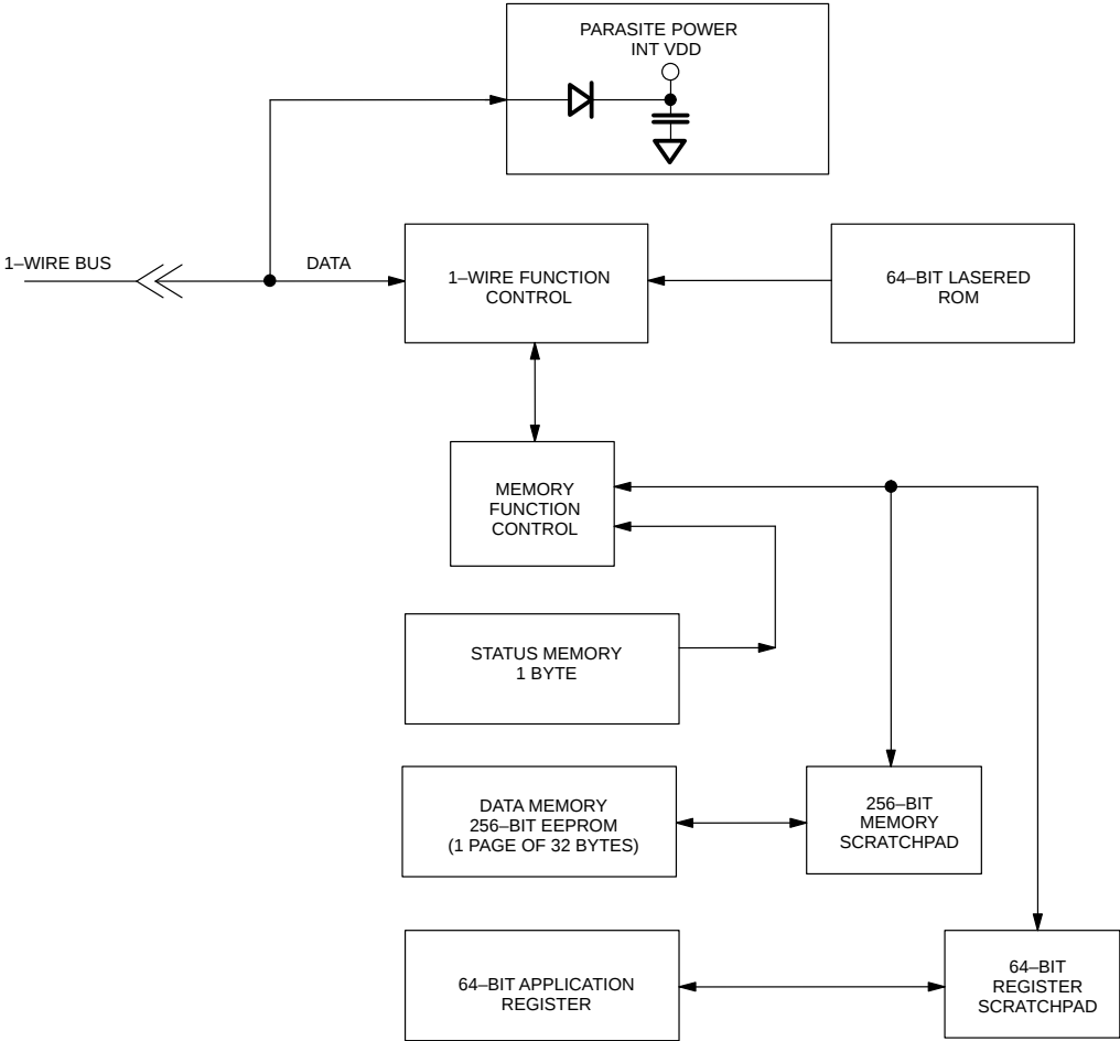
DS2430A BLOCK DIAGRAM Figure 1
