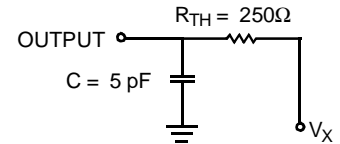
(c) Three-State Delay (Load 1)
