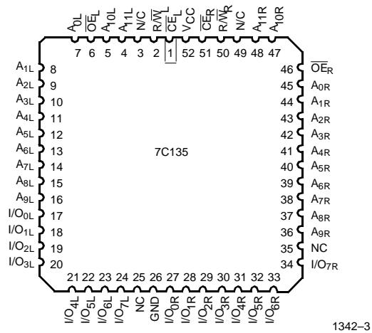
PLCC Top View
