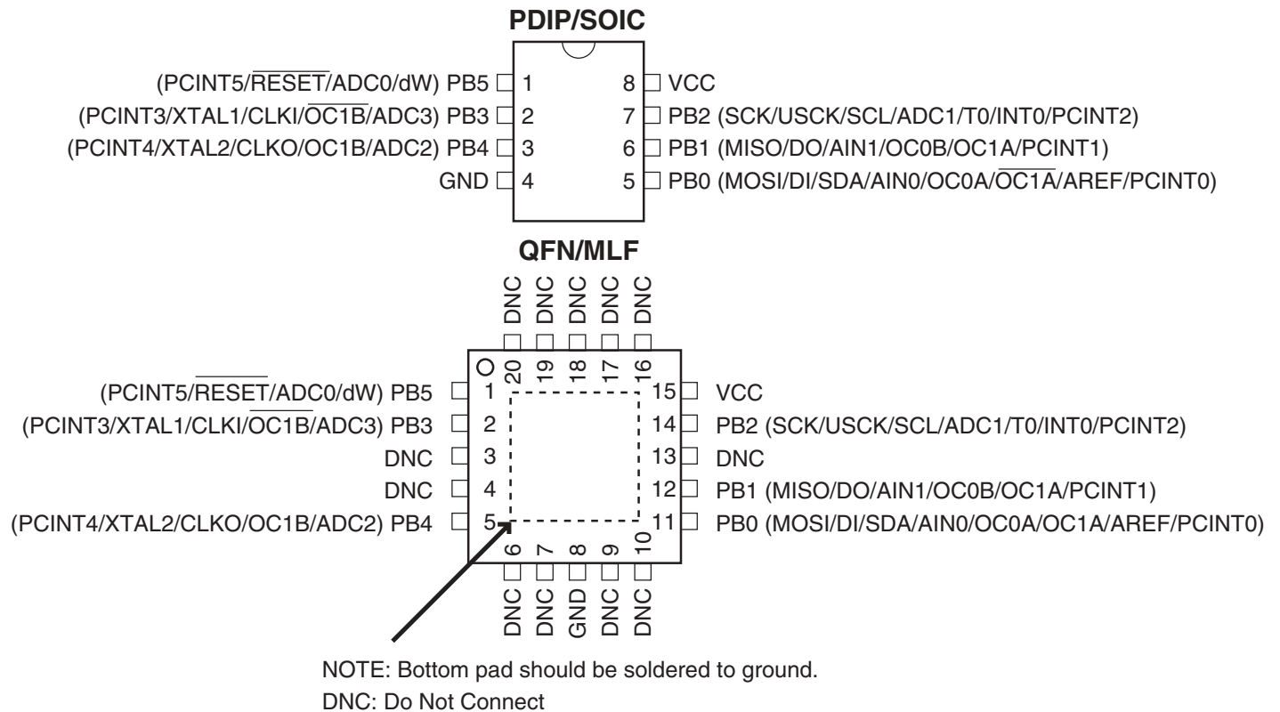
Figure 1-1. Pinout ATtiny25/45/85
