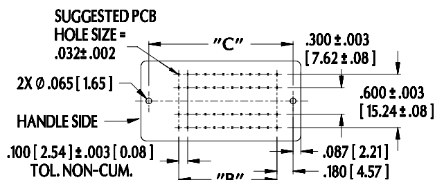
SOCKET FOOTPRINT (top view - component side)
