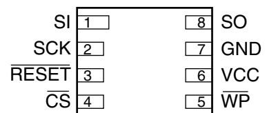
Figure 2-4. CASON – Top View through Package
