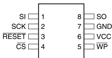
Figure 2-3. SOIC Top View
