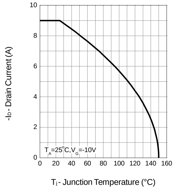
Drain Current
