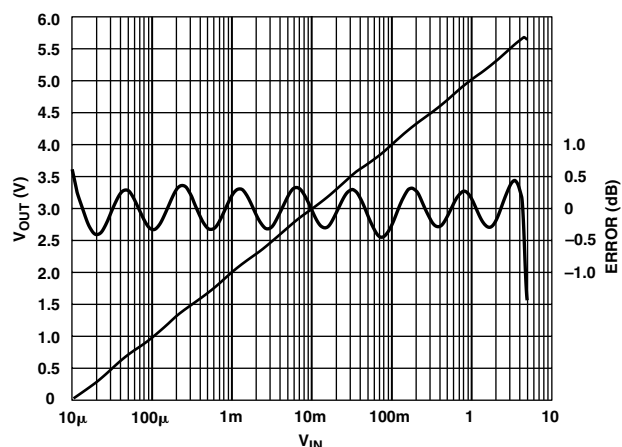
Figure 26. Ideal Output and Law-Conformance Error for the DC-Coupled AD8307 at 50 mV/dB
