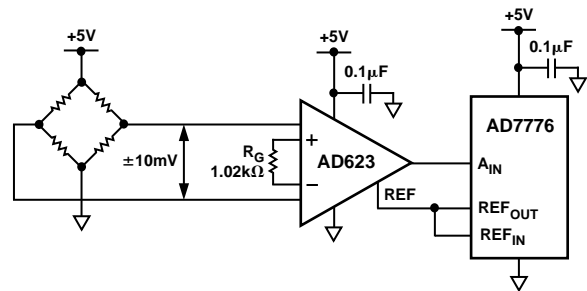
Figure 49. A Single Supply Data Acquisition System
