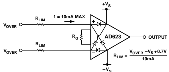
Figure 42. Input Protection
