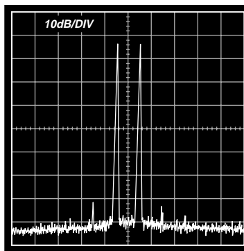
Figure 23. Third Order Intermodulation Distortion at 10.7 MHz (10x Probe Used to HP3585A Spectrum Analyzer, Gain = 0 dB, P_{IN} = 0 dBm, Pin 5 Connected to Pin 7)
