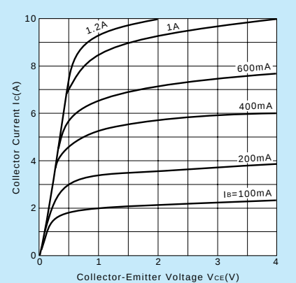
I c -V CE Characteristics (Typical)
