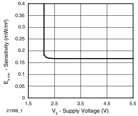
21398_1 Fig. 13 - Sensitivity vs. Supply Voltage
