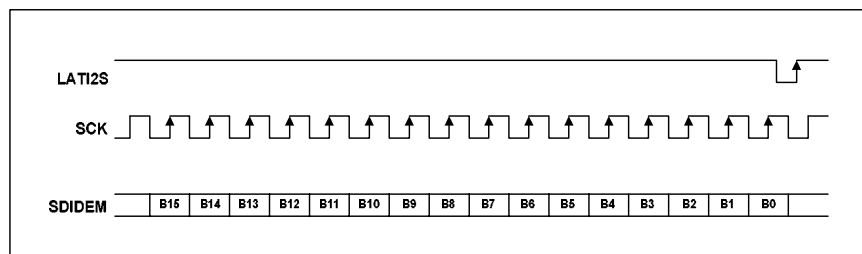
Figure 13 3-Wire Serial Interface
