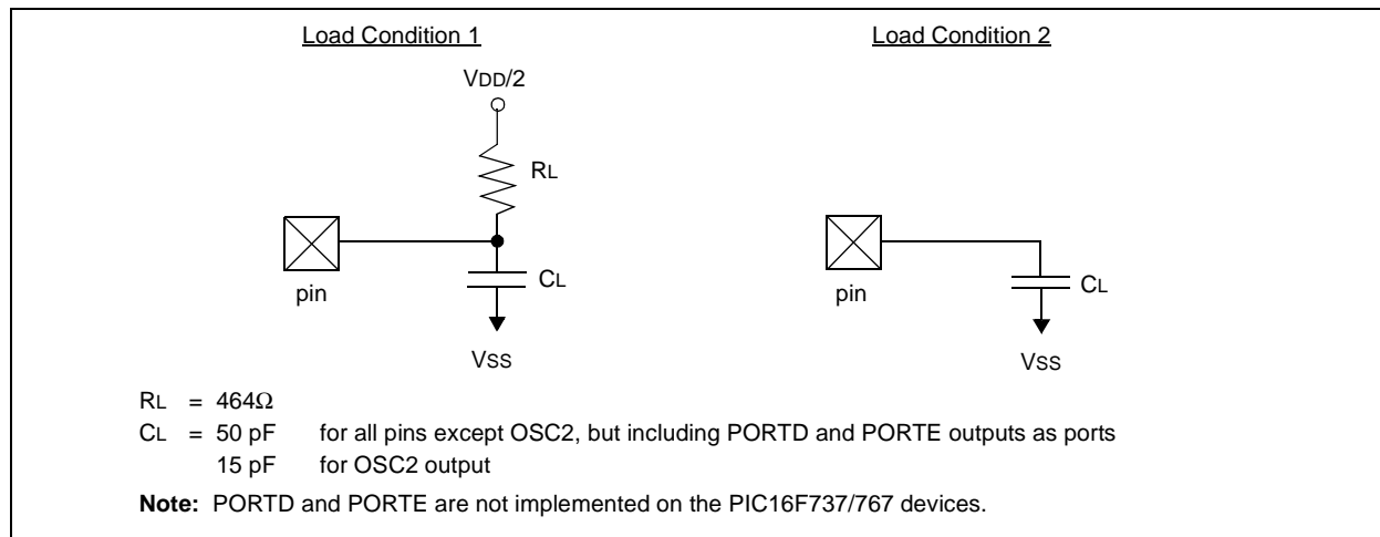
FIGURE 18-4: LOAD CONDITIONS
