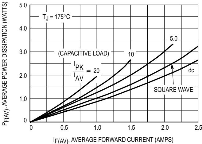
Figure 9. Power Dissipation
