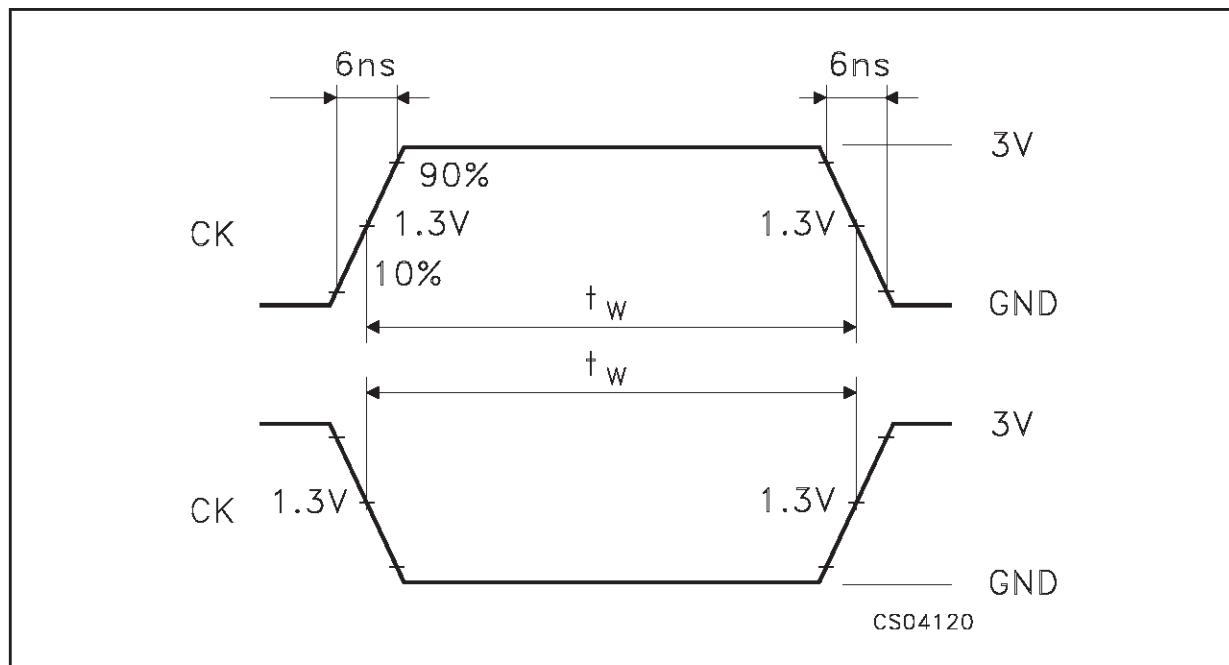
WAVEFORM 3 : MINIMUM PULSE WIDTH (f=1MHz; 50% duty cycle)
